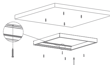
2. Knock the plastic anchor into ceiling, fix the surface mounted frame on the ceiling by screws.
