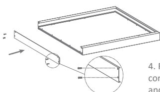
1. Assemble the surface mounted frame and fix by screws.
