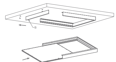
3. Fix the side frame back by screw.
