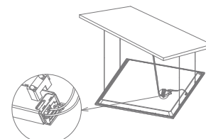
3. Adjust the length of steel wire. Connect the power supply.
