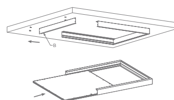
3. Fix the side frame back by screw.
