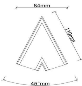
45D corner
