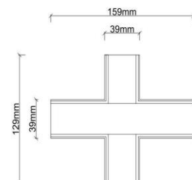
Cross
