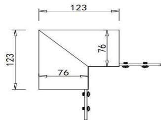
Outer corner
